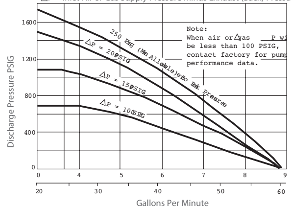
Capacity Data Model 6121 Pump
