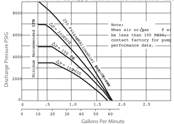
Capacity Data Model 6111 Pump
