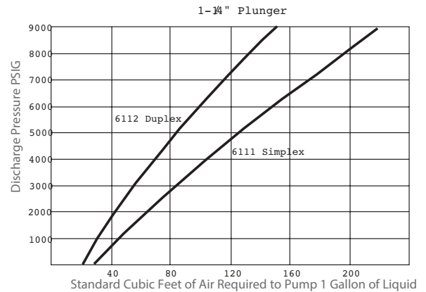
Capacity Data Model 6111 Pump
